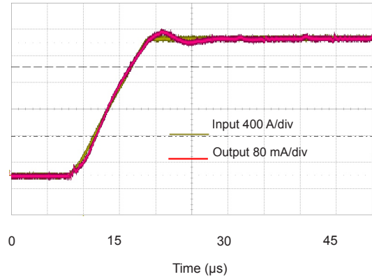
Figure 2: Typical step response (0 to 2 kA, 400 A/μs)
