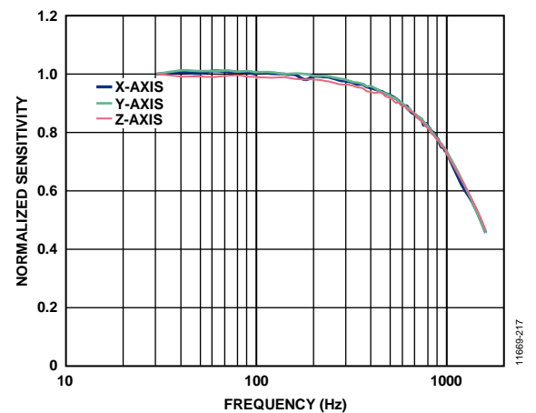
Figure 21. Frequency Response
