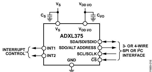
Figure 31. Application Diagram
