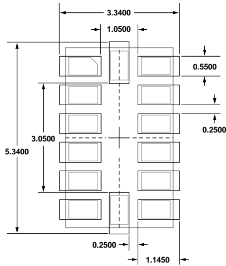
Figure 38. Recommended Printed Wiring Board Land Pattern (Dimensions shown in millimeters)
