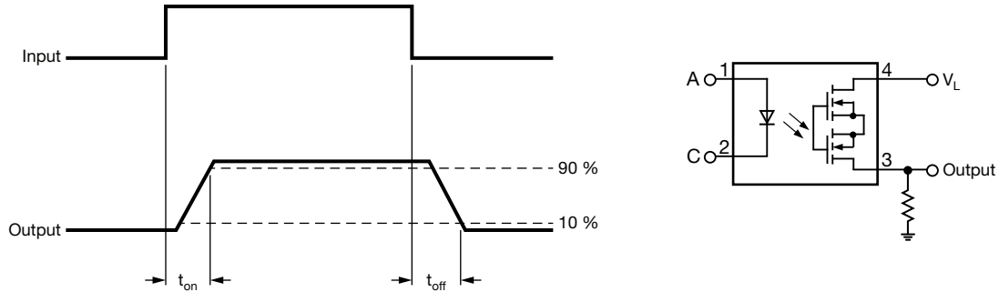
Fig. 1 - Timing Schematic
