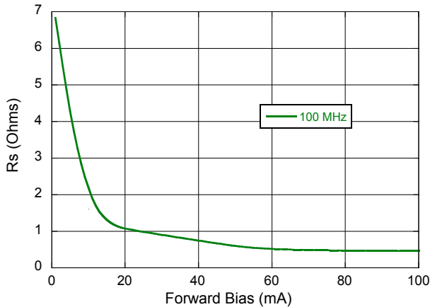
Series Resistance vs. Forward Current
