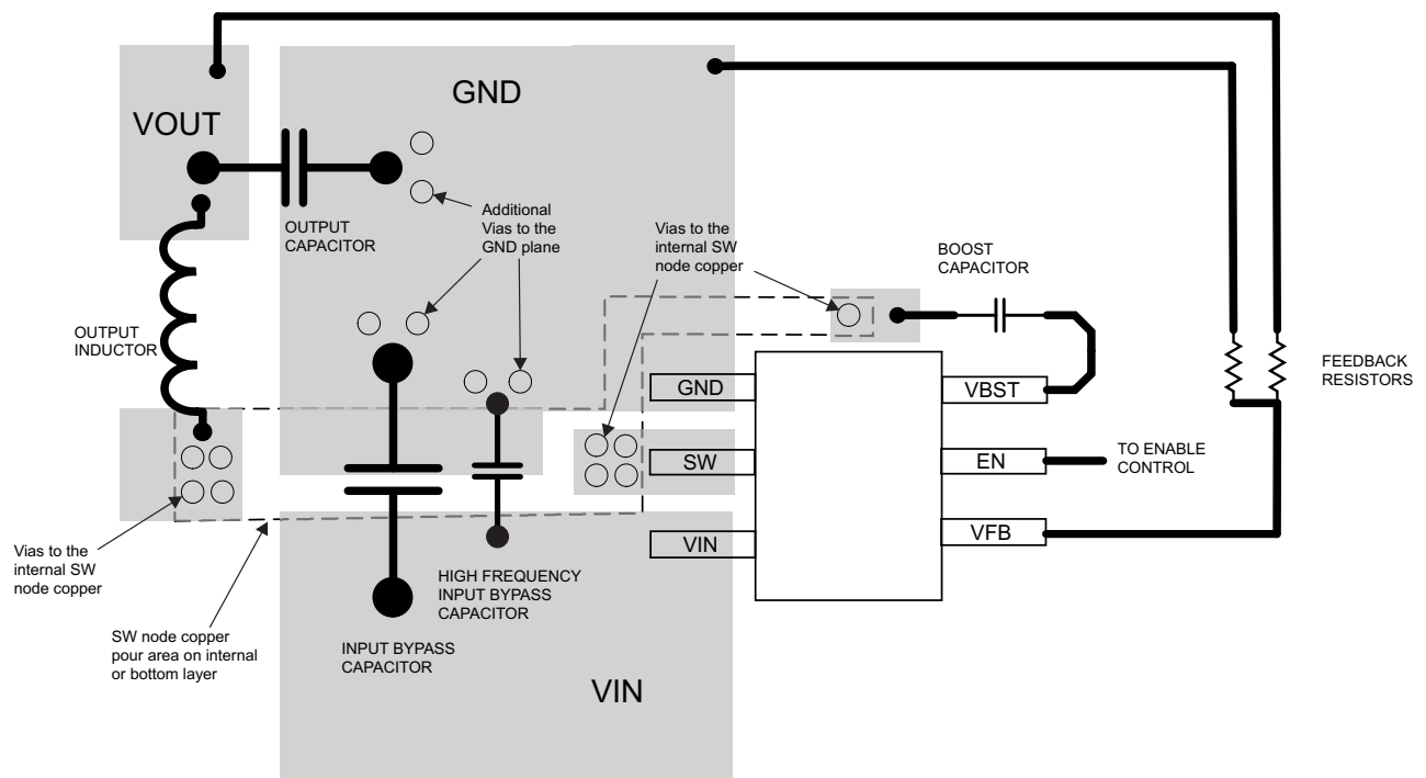
Figure 50. Typical Layout
