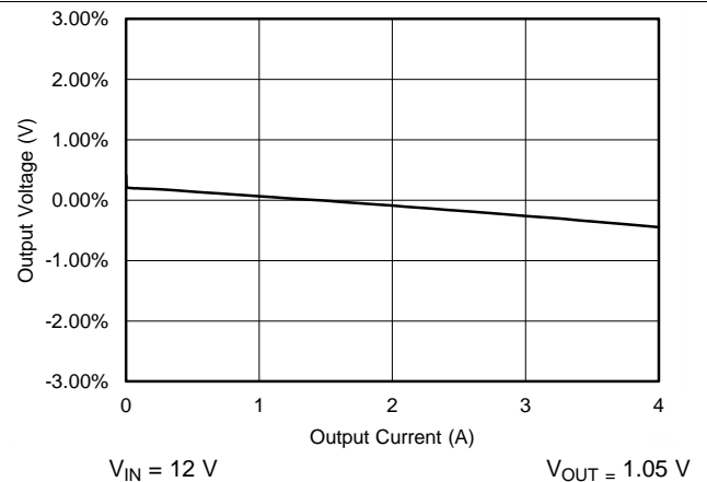
Figure 16. Load Regulation, V_{IN} = 12\text{ V}
