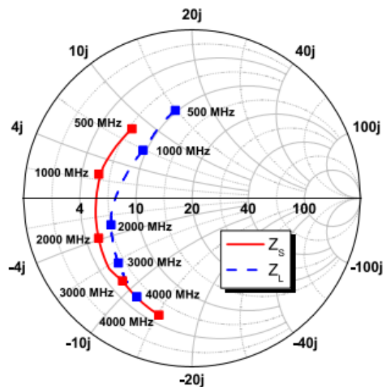
Figure 3 - Optimum Impedances for CW Performance, V_{DS} = 28\text{ V}
