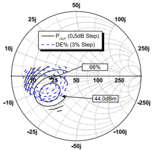
Figure 7 - Load-Pull Contours, 2500MHz, P_{IN} = 29.4\text{dBm} , Z_S = 4.8 - j3.0\ \Omega
