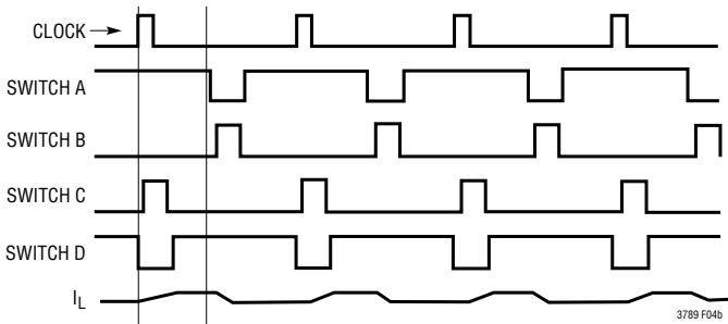
(4b) Buck-Boost Region ( V_{\text{IN}} \leq V_{\text{OUT}} )
