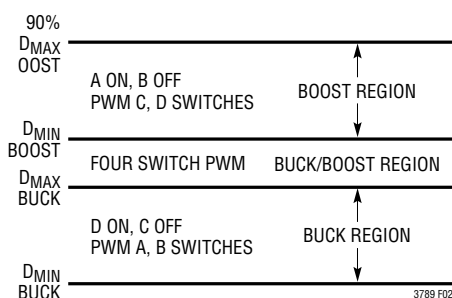
Figure 2. Operating Region vs Duty Cycle
