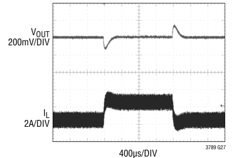
Load Step
