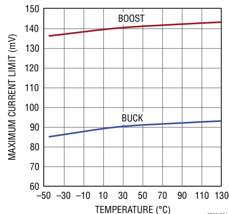
Maximum Current Limit vs Temperature
