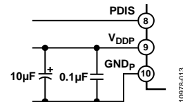
Figure 16. V_{DDP} Bias and Bypass Components
