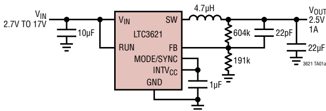
2.5V V_{OUT} with 400mA Burst Clamp, f_{SW} = 1MHz
