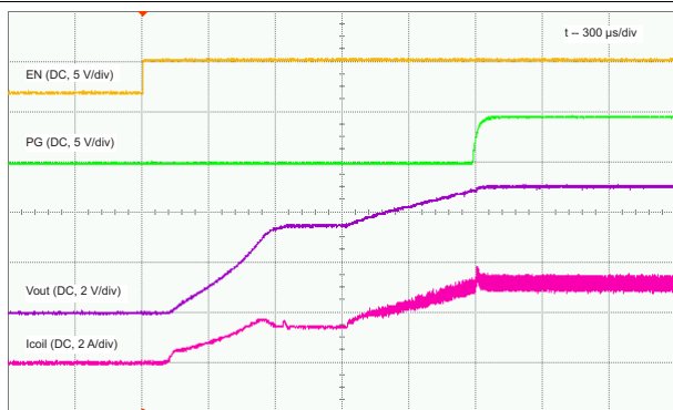
Figure 23. Startup ( V_{OUT} = 5\text{ V} , R_{OUT} = 2.5\ \Omega )
