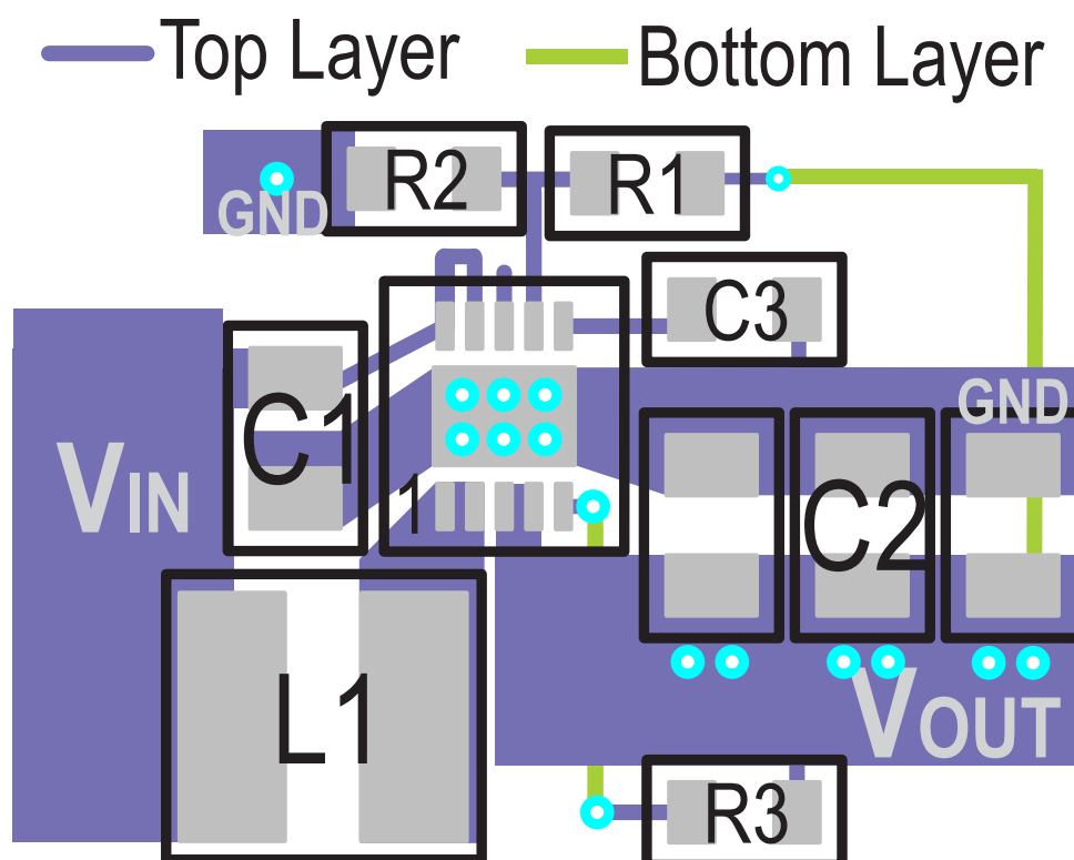
Figure 37. Layout Recommendation
