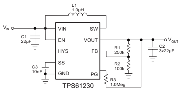
Figure 25. TPS61230 3.5-V Output Typical Application
