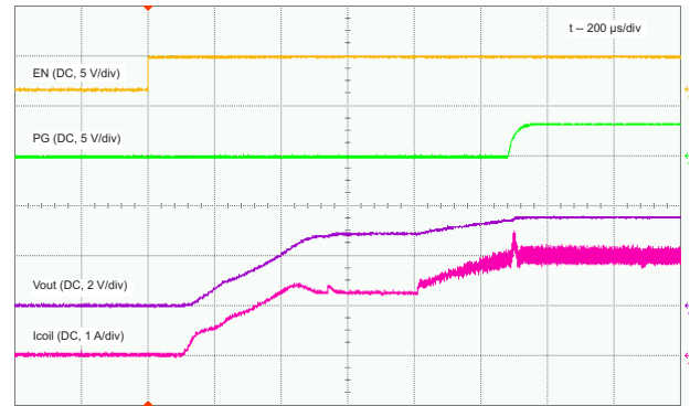
Figure 33. Startup ( V_{OUT} = 3.5\text{ V} , V_{IN} = 3.0\text{ V} , R_{OUT} = 2.3\ \Omega )
