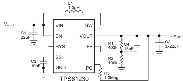
Figure 35. TPS61230 5-V Output with Cff Typical Application
