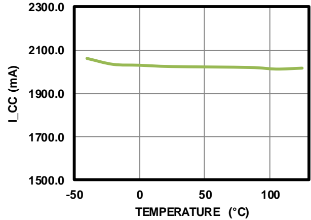
VCC Leakage Current @ 28V vs. Temperature
