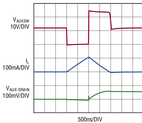
Auxiliary Boost Regulator Switching Waveforms
