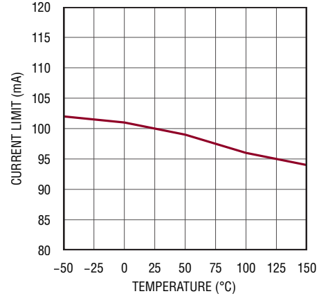
Auxiliary Boost Regulator Current Limit
