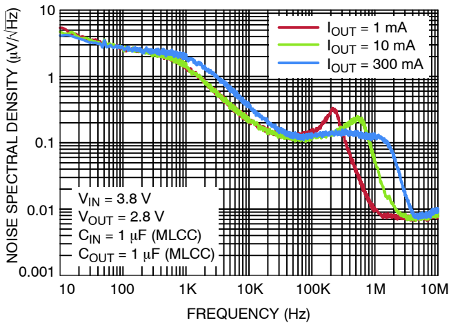
Figure 22. Output Voltage Noise Spectral Density – V_{OUT} = 2.8 \text{ V}
