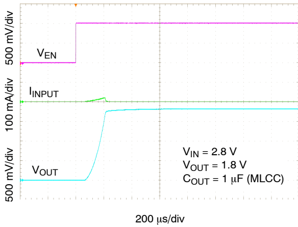
Figure 28. Enable Turn-on Response – I_{OUT} = 0 \text{ mA} , Slow Option – C
