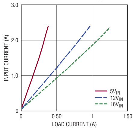
Input vs Load Current, V_{OUT} \pm 12V
