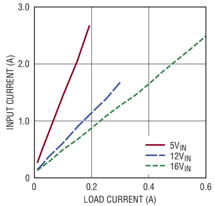
Input vs Load Current, V_{OUT} \pm 24V
