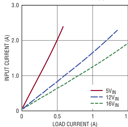
Input vs Load Current, V_{OUT} \pm 8V
