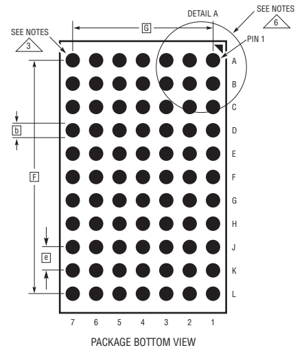
PACKAGE BOTTOM VIEW
