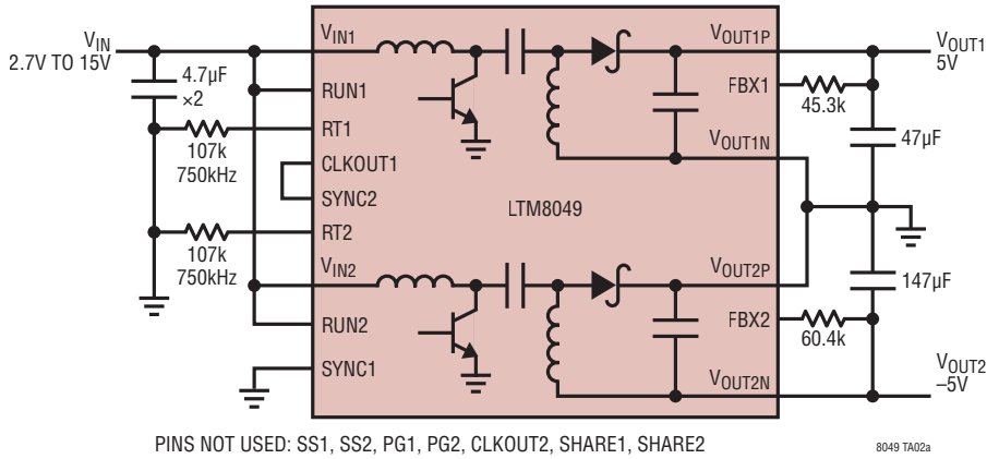
±5V Converter
