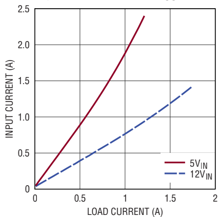
Input vs Load Current, V_{OUT} \pm 3.3V
