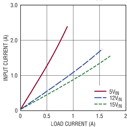
Input vs Load Current, V_{OUT} \pm 5V
