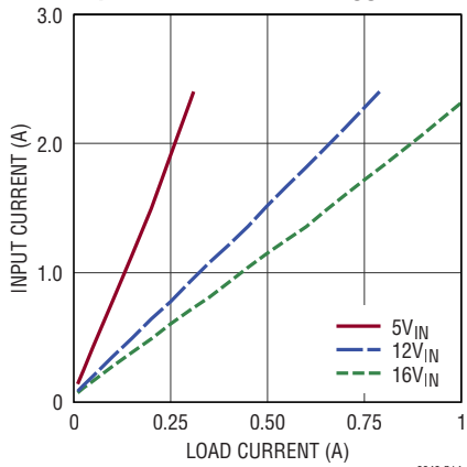
Input vs Load Current, V_{OUT} \pm 15V
