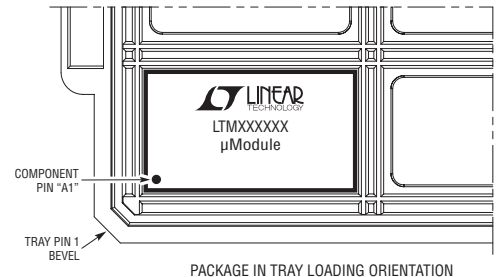
PACKAGE IN TRAY LOADING ORIENTATION
