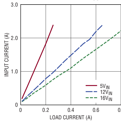
Input vs Load Current, V_{OUT} \pm 18V
